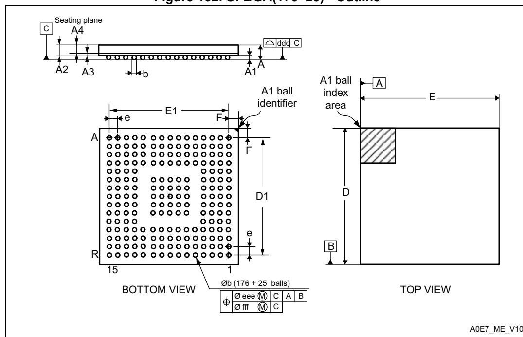
Figure 132. UFBGA(176+25) - Outline
