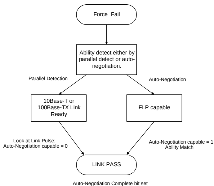
Figure 10. Auto-Negotiation and Parallel Detect
