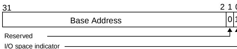
Figure 17. Base Address Register for I/O Mapping
