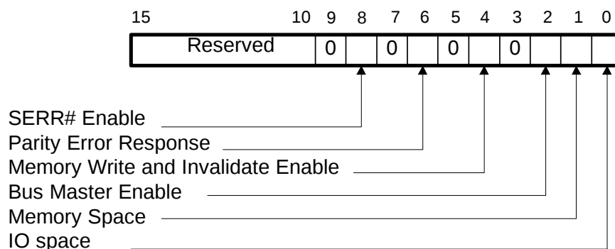
Figure 13. PCI Command Register
