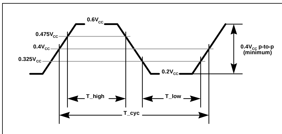
Figure 21. PCI Clock Waveform
