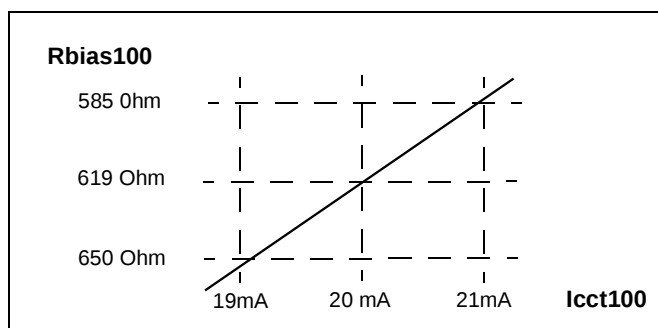
Figure 19. RBIAS100 Resistance Versus Transmitter Current
