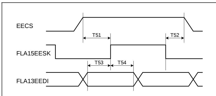
Figure 26. EEPROM Timings
