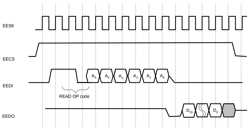
Figure 9. 64-Word EEPROM Read Instruction Waveform
