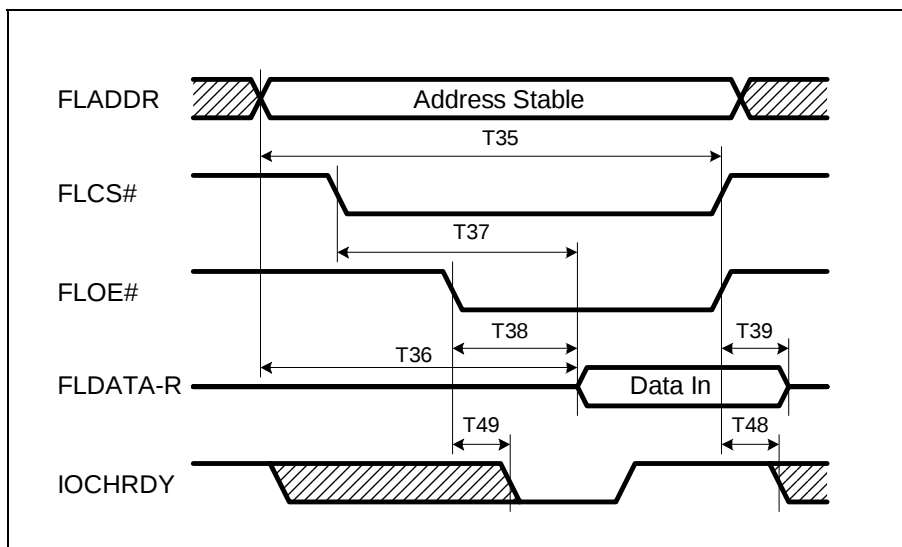
Figure 24. Flash Timings for a Read Cycle
