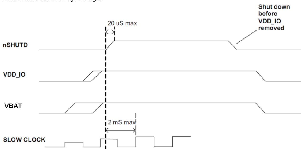
Figure 4 Bluetooth Power-Up/Down Sequence
