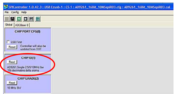
Figure 6. AD9261 SPIController
