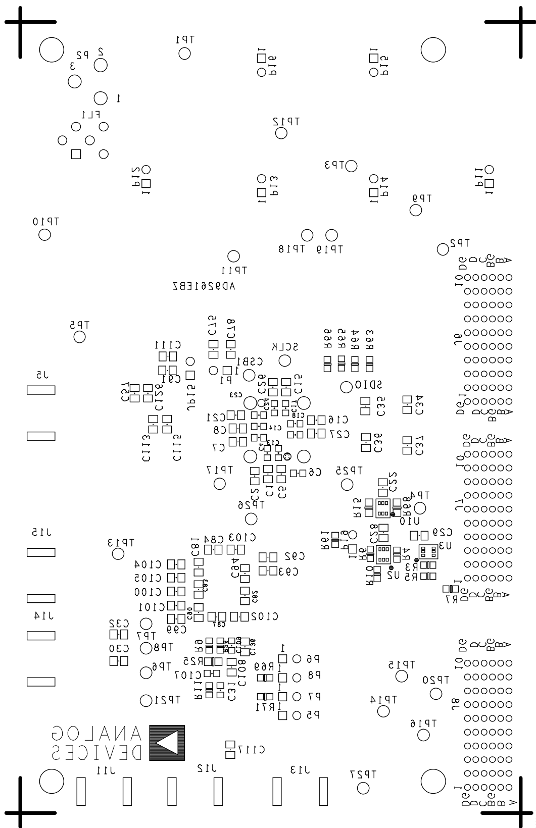
Figure 19. Bottom Silk
