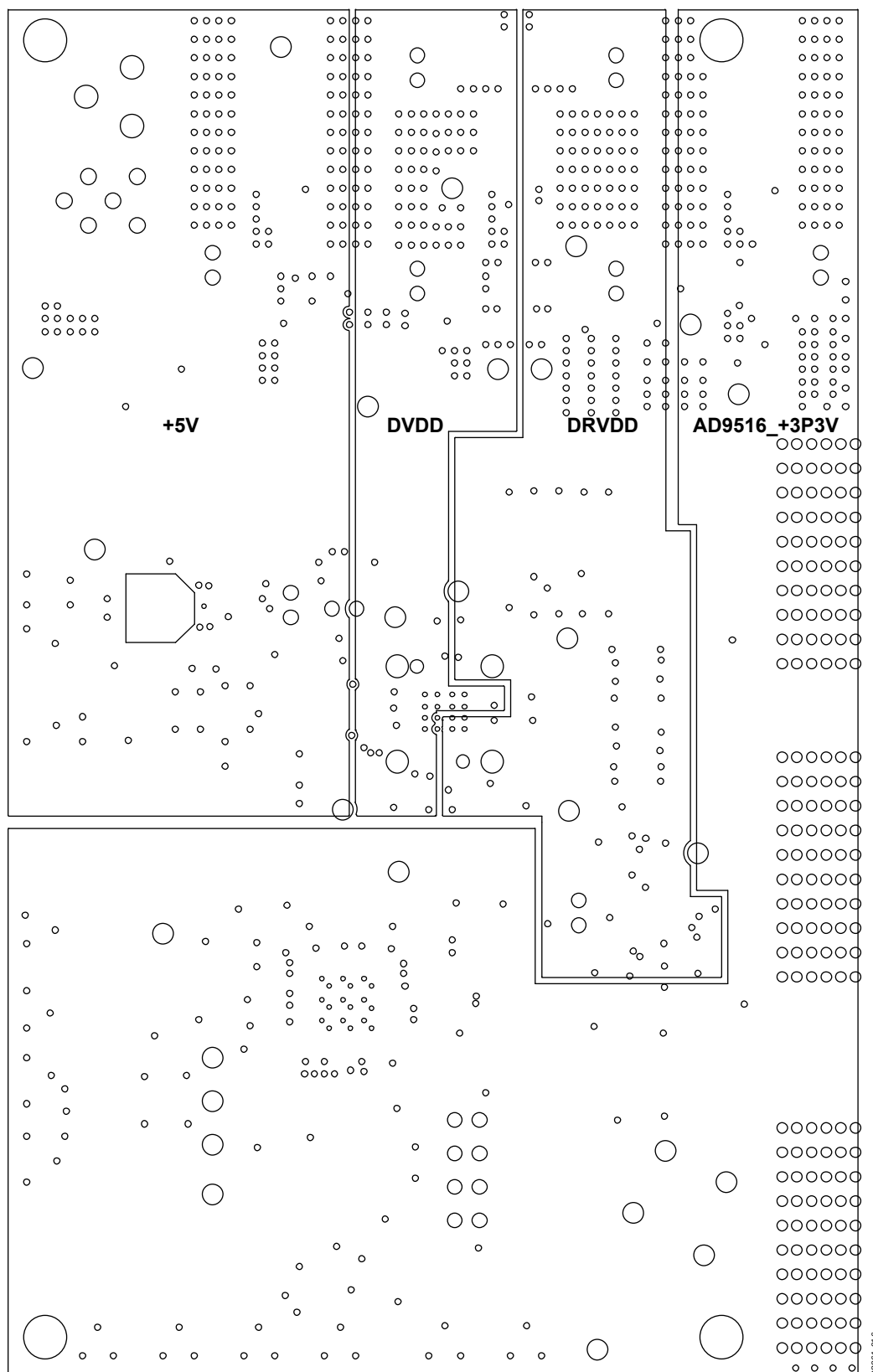
Figure 21. Power Layer 4
