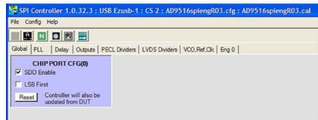
Figure 9. AD9516 Configuration
