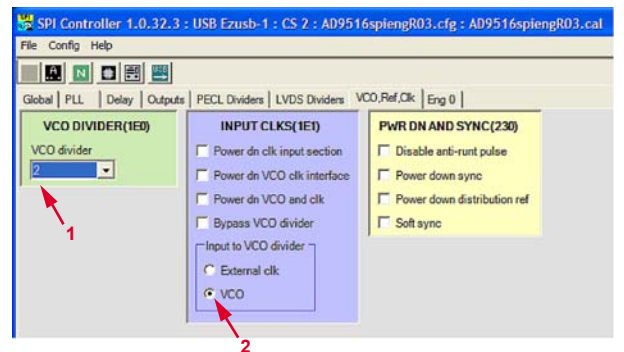
Figure 10. VCO and Clock Configuration for the 122.88 MHz Crystal Oscillator
