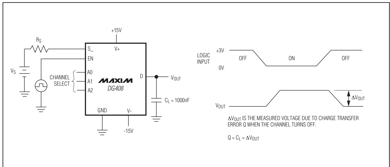
Figure 5. Charge Injection
