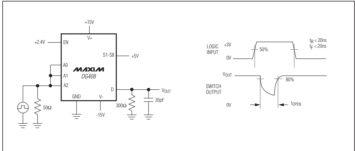
Figure 4. Break-Before-Make Interval
