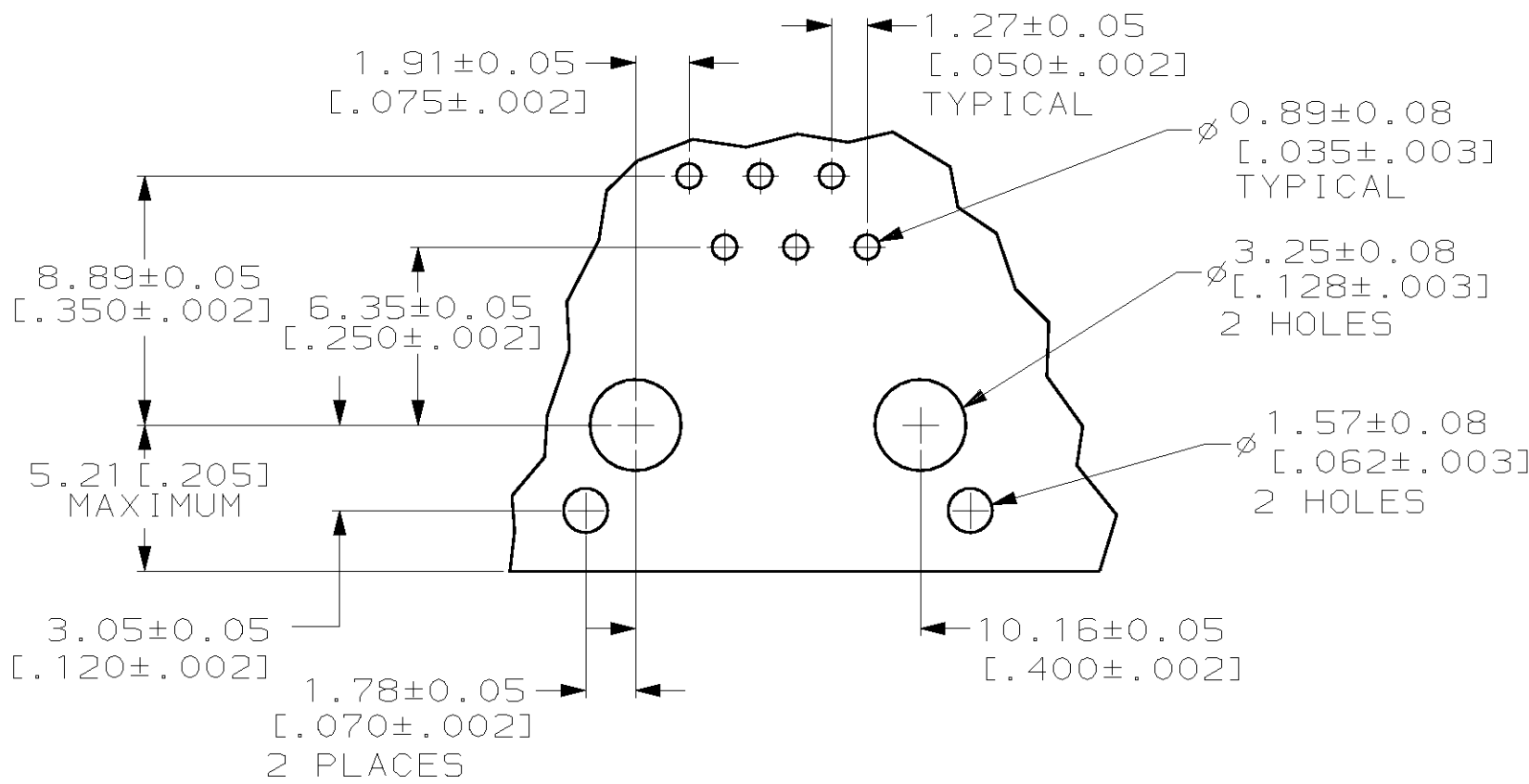
SUGGESTED PRINTED CIRCUIT BOARD MOUNTING HOLE LAYOUT VIEW SHOWN AS COMPONENT SIDE OF BOARD
