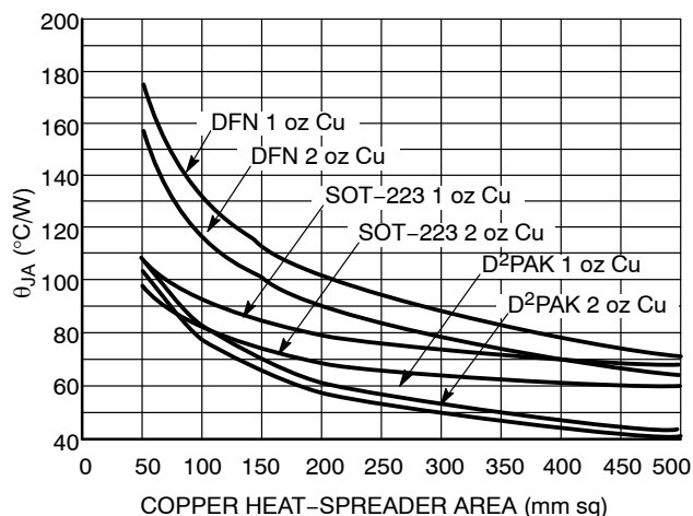
Figure 25. Thermal Resistance
