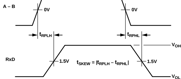
Figure 36. Receiver Propagation Delay
