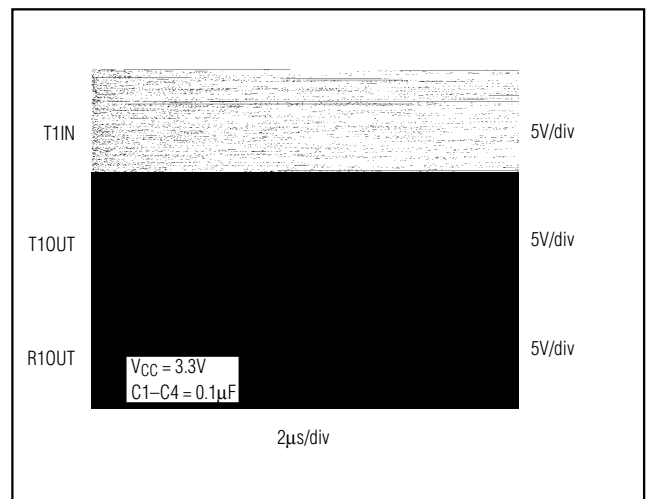
Figure 8. MAX3384E Loopback Test Result at 250kbps
