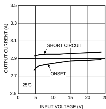
Figure 28. Current Limit, V_{OUT} = 3.3\text{ V}
