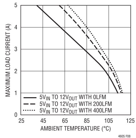
Figure 8. 5V IN to 12V OUT with Heatsink
