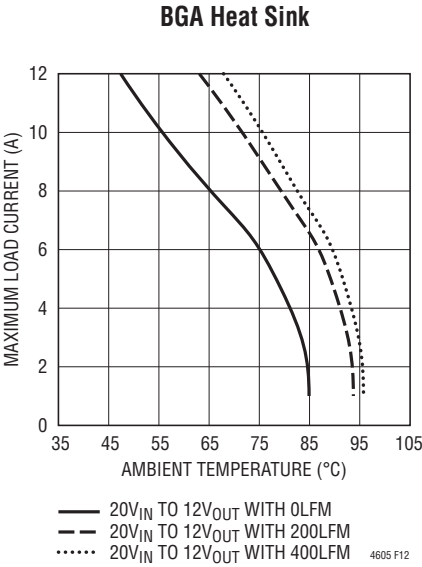
Figure 12. 20V IN to 12V OUT with Heatsink
