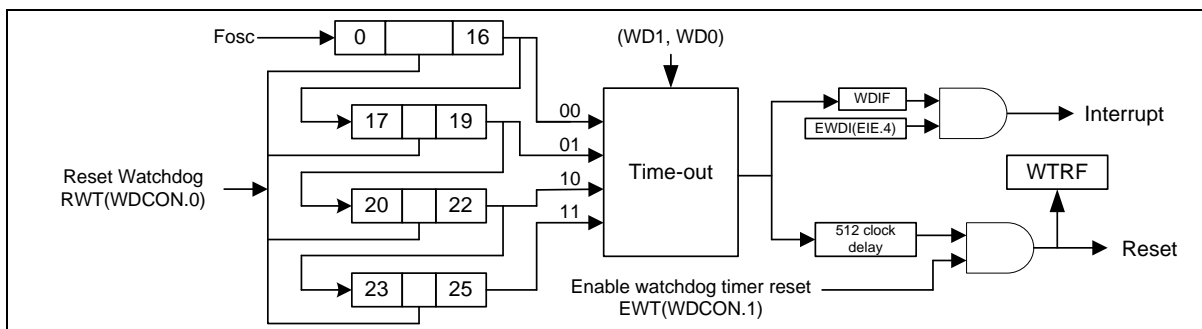
Figure 12-1 Watchdog Timer
