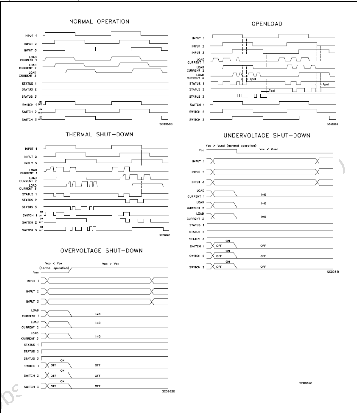
Figure 6. Switching waveforms
