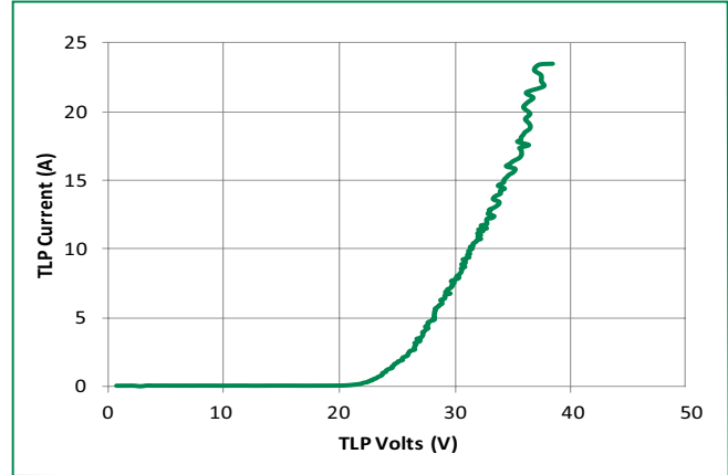
Transmission Line Pulsing (TLP) Plot (Pin 1 to Pin2)
