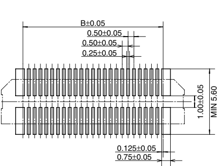
Recommended PC board pattern (TOP VIEW)
