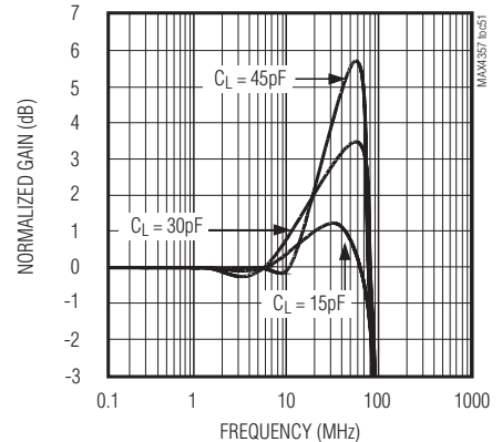
MEDIUM-SIGNAL FREQUENCY RESPONSE ( A_V = +2V/V )
