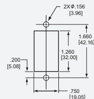
Mounting Detail Single, Two & Three Pole
