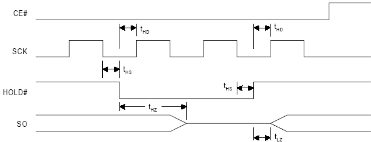
Figure 32. HOLD TIMING
