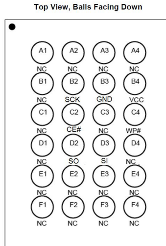
TFBGA-24 (Package: JG)
