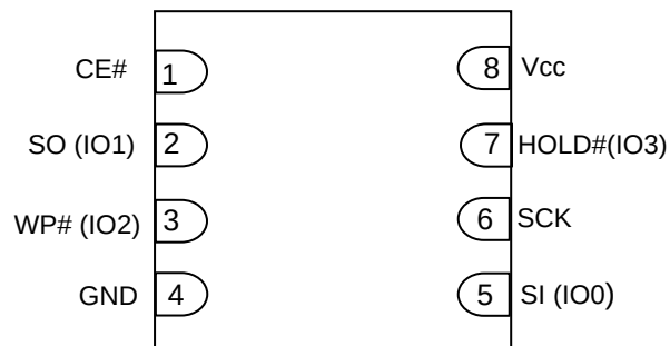
8-pin WSON 6x5mm (Package: JK) 8-pin WSON 8x6mm (Package: JL)
