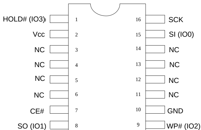
SOIC-16 300mil (Package: JM)
