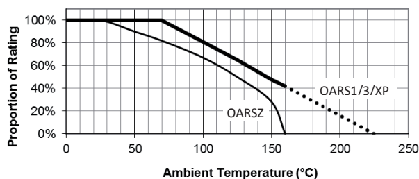
Temperature Derating
