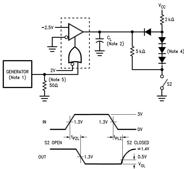
Figure 2. t_{PHZ} , t_{PZH}
