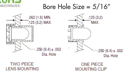
PH25 Mounting
