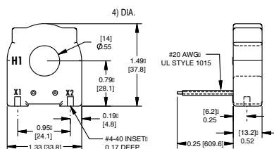
Model 18 Dimensions
