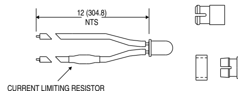
PH25 Outline
