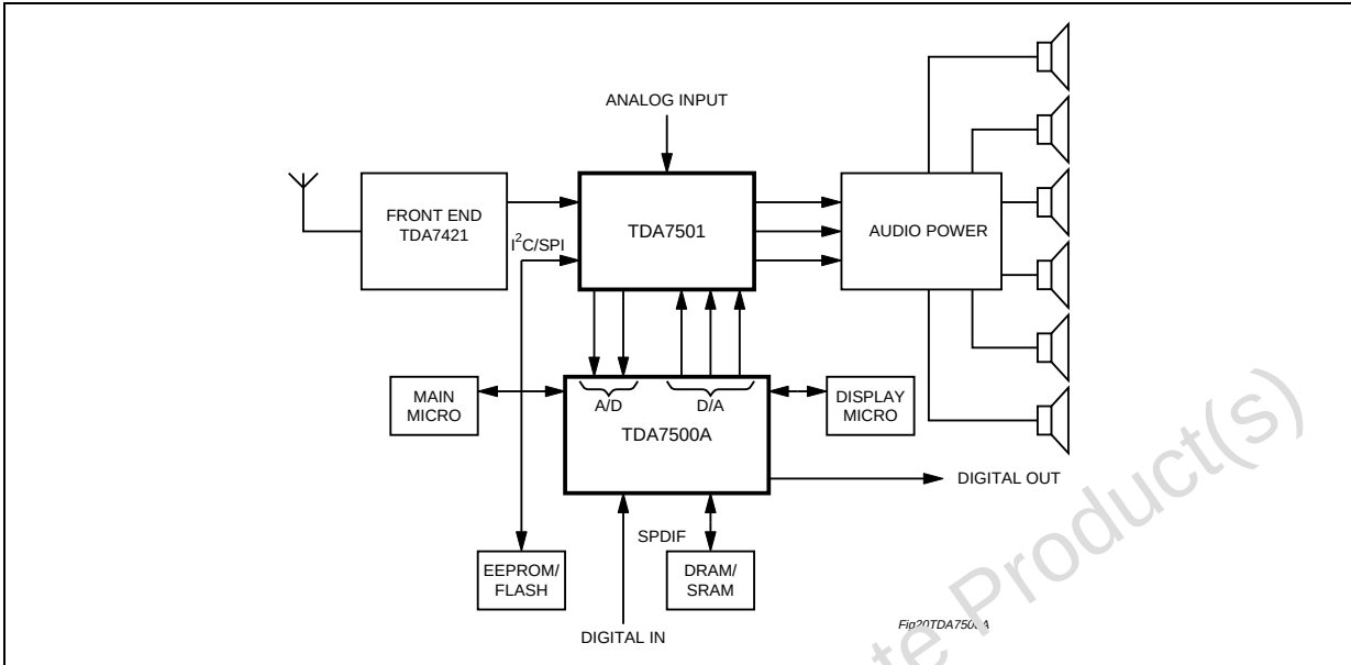
Figure 20. block Diagram of Car Amplifier Audio Sub-System.
