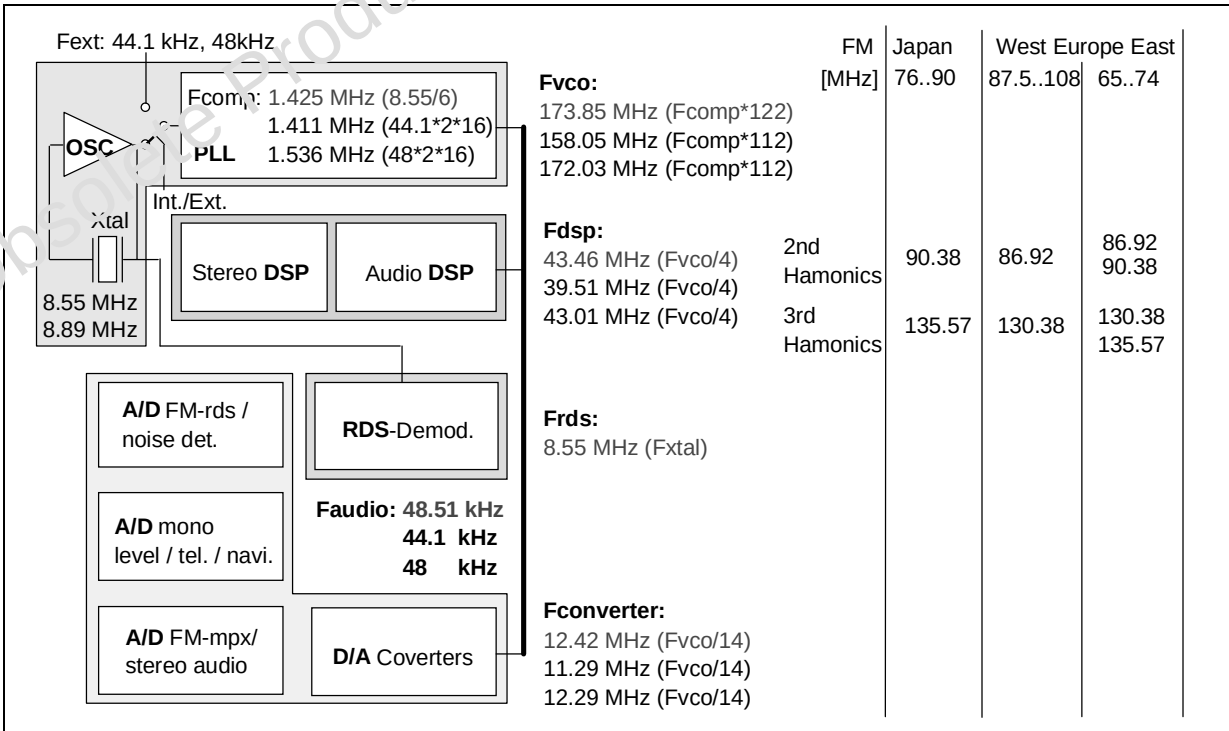
Figure 21. Clock Scheme
