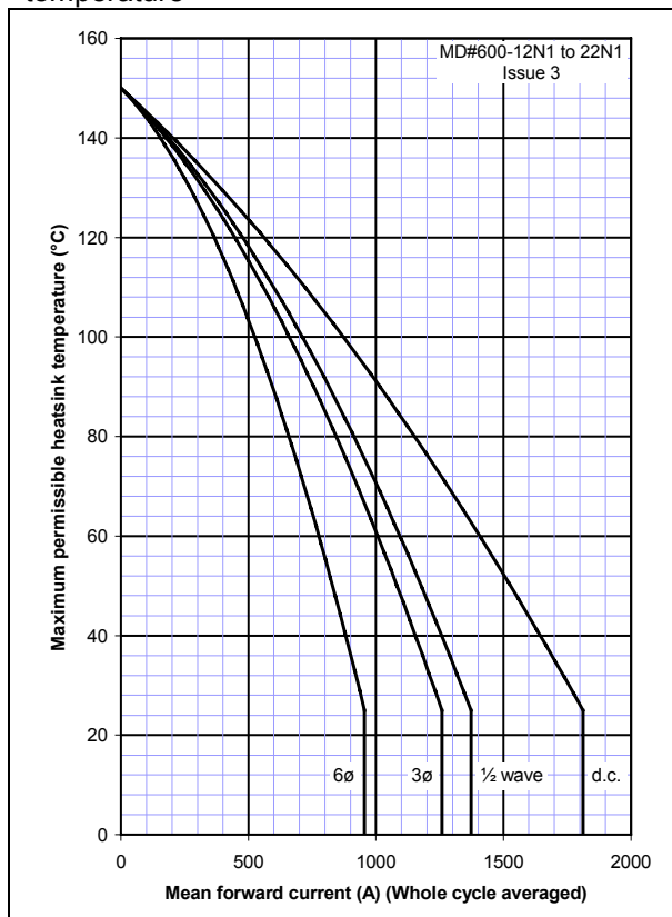
Figure 8 – Forward current vs. Heatsink temperature
