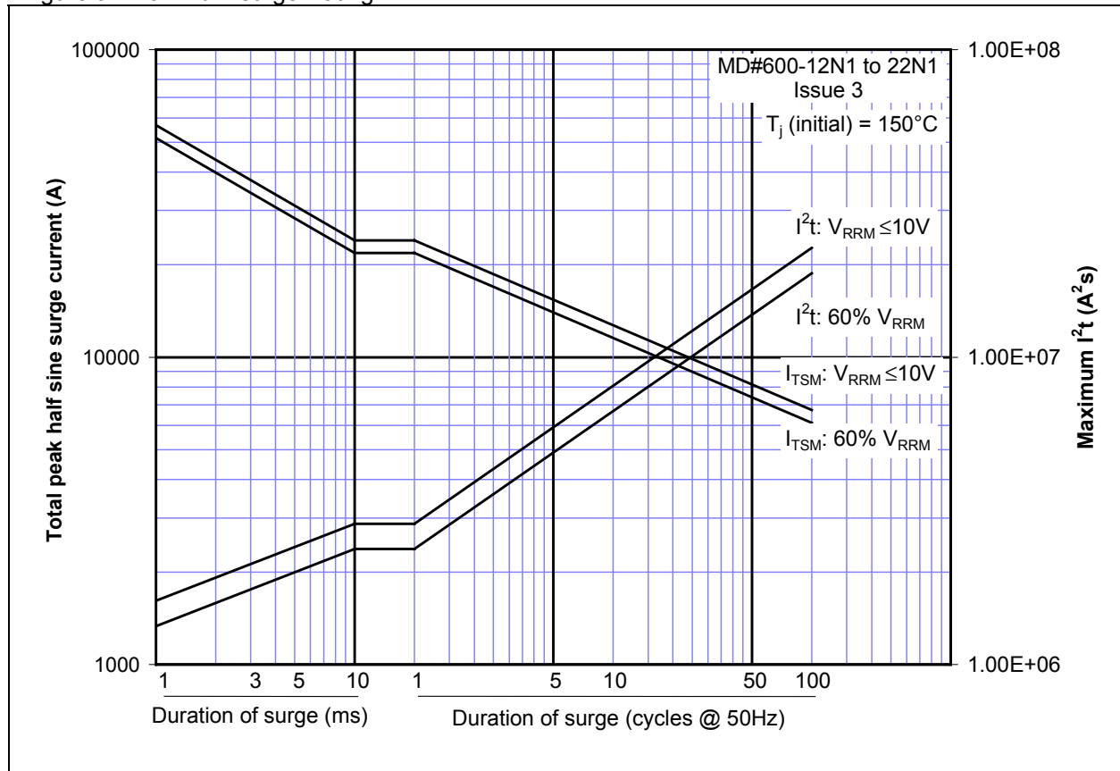
Figure 9 - Maximum surge Rating
