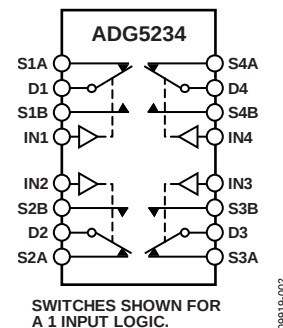
Figure 2. ADG5234 TSSOP and LFCSP_WQ
