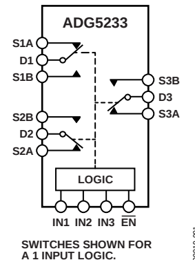
Figure 1. ADG5233 TSSOP and LFCSP_WQ
