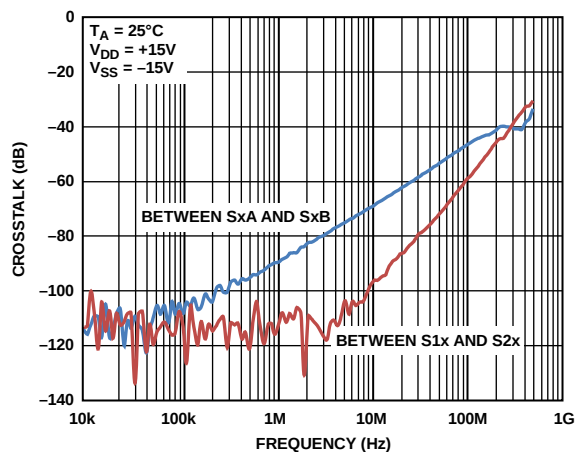
Figure 20. Crosstalk vs. Frequency, ±15 V Dual Supply
