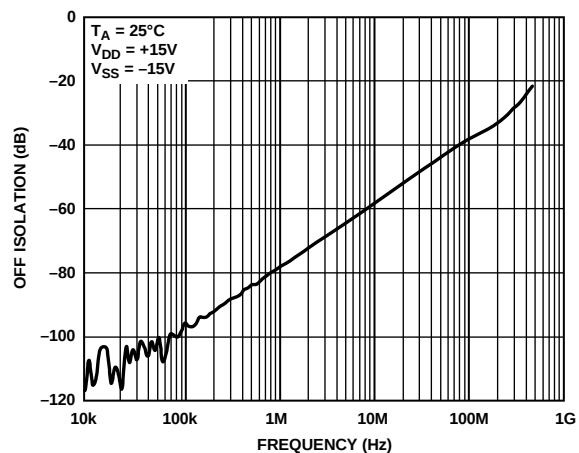
Figure 19. Off Isolation vs. Frequency, ±15 V Dual Supply
