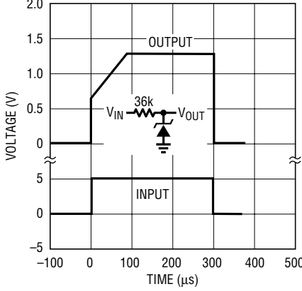
Response Time
