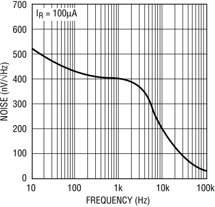
Noise Voltage
