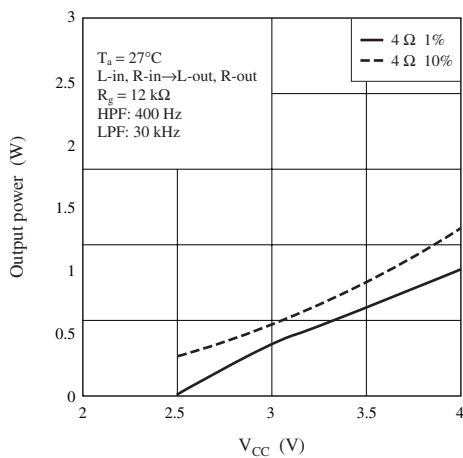
R-ch. 4 \Omega
