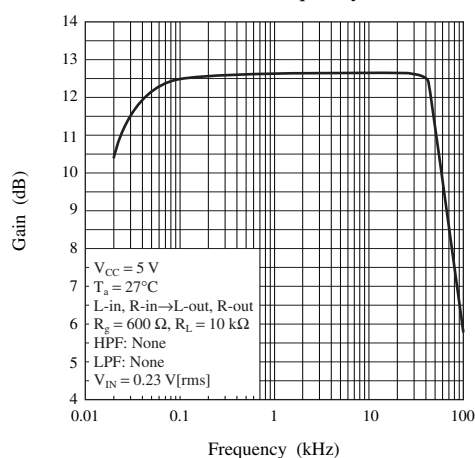
Gain — Frequency
