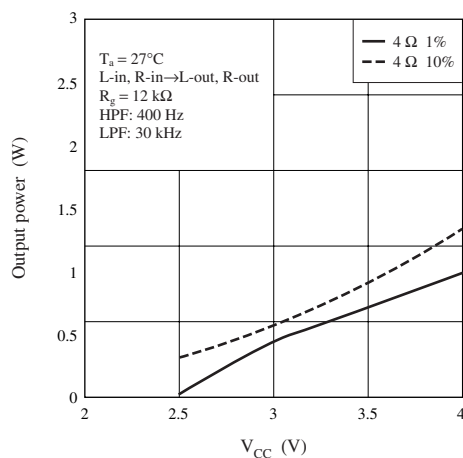
L-ch. 4 \Omega
