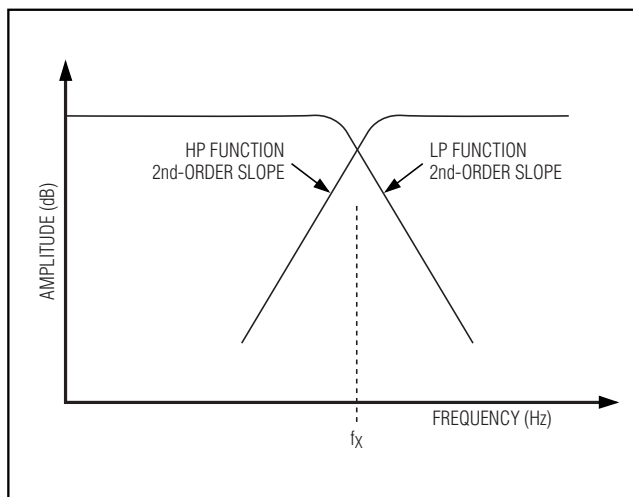
Figure 6. Crossover Frequency
