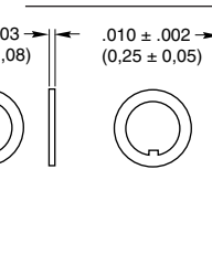
Keyed Washer
