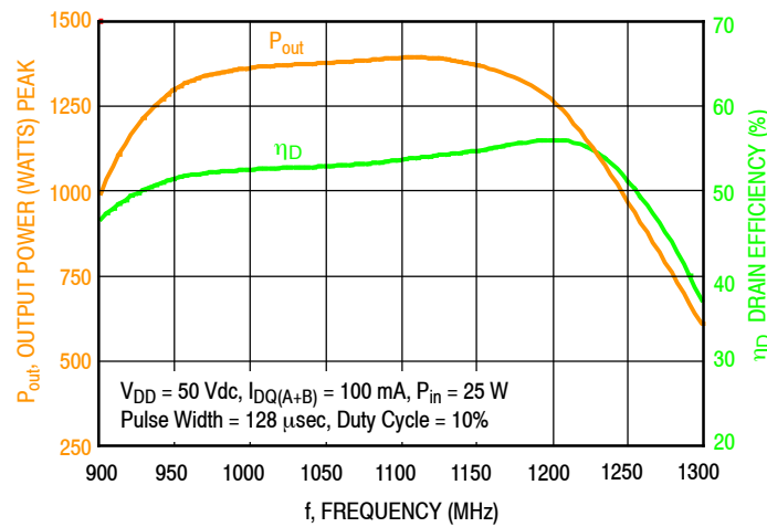
Figure 8. Output Power and Drain Efficiency versus Frequency at a Constant Input Power
