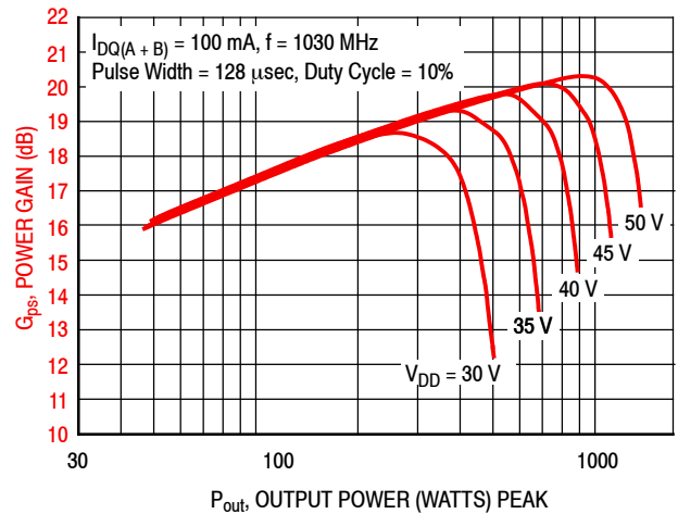
Figure 14. Power Gain versus Output Power
