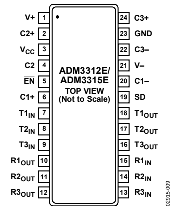
Figure 9. SSOP/TSSOP Pin Configuration
