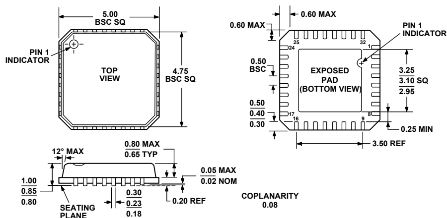
COMPLIANT TO JEDEC STANDARDS MO-220-VHHD-2 Figure 37. 32-Lead Lead Frame Chip Scale Package [LFCSP_VQ] 5 mm x 5 mm Body, Very Thin Quad (CP-32-2) Dimensions shown in millimeters
