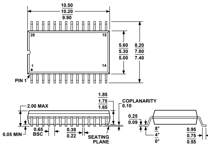
COMPLIANT TO JEDEC STANDARDS MO-150-AH Figure 38. 28-Lead Shrink Small Outline Package [SSOP] (RS-28) Dimensions shown in millimeters
