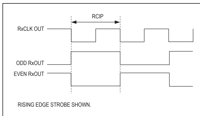
Figure 2. Worst-Case Test Pattern
