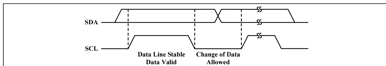
Figure 3 Bit transfer
