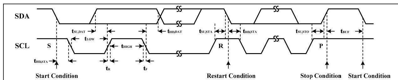
Figure 2 Interface timing
