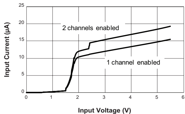
Quiescent Current
