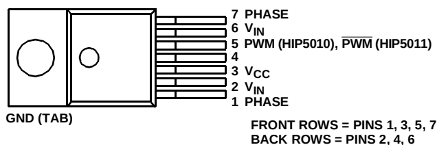
HIP5010IS1, HIP5011IS1 (SIP - VERTICAL) TOP VIEW
