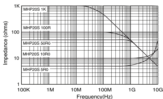
Frequency Characteristics
