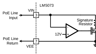
Figure 9. Detection Circuit With Integrated PD Signature Resistor
