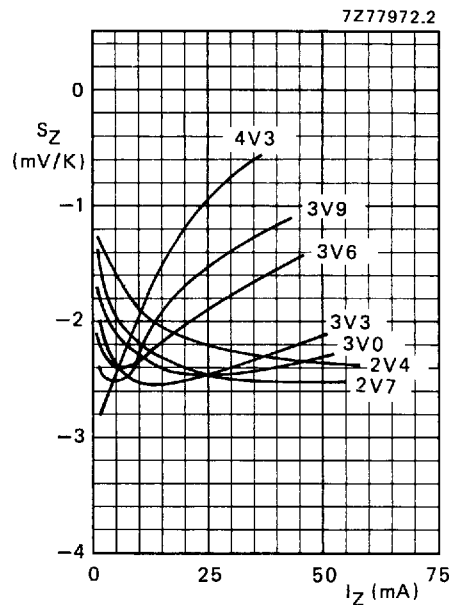
Fig. 14 Typical values; T_j = 25\text{ to }150\text{ °C} .
