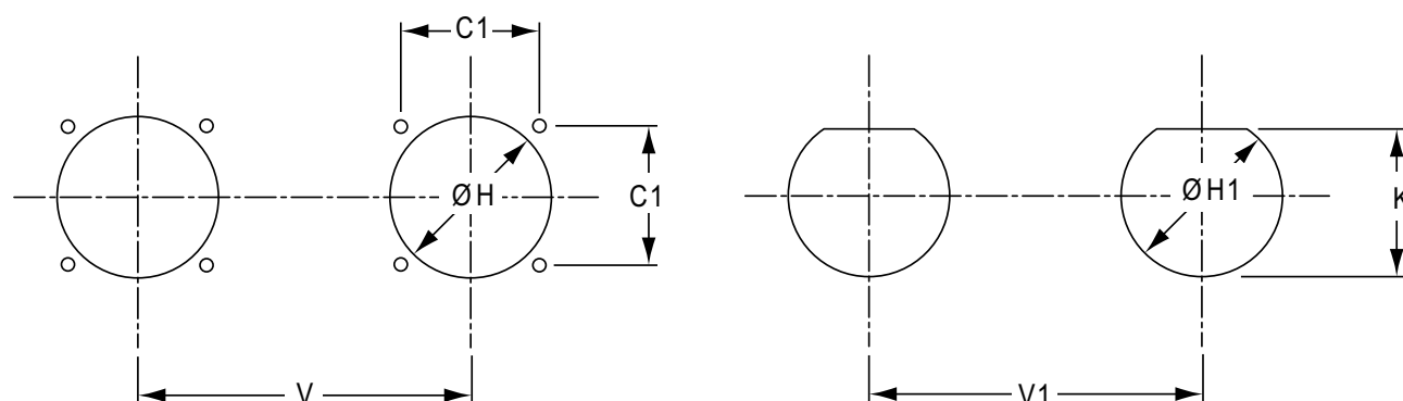
Square Flange Receptacle (Type 20)
