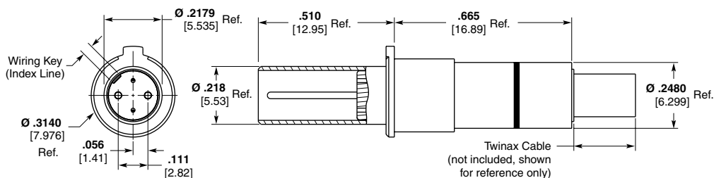
Part No. 1811865-1
