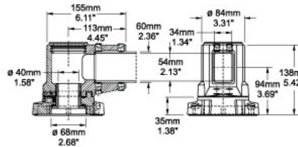
Front Section Socket Joint
