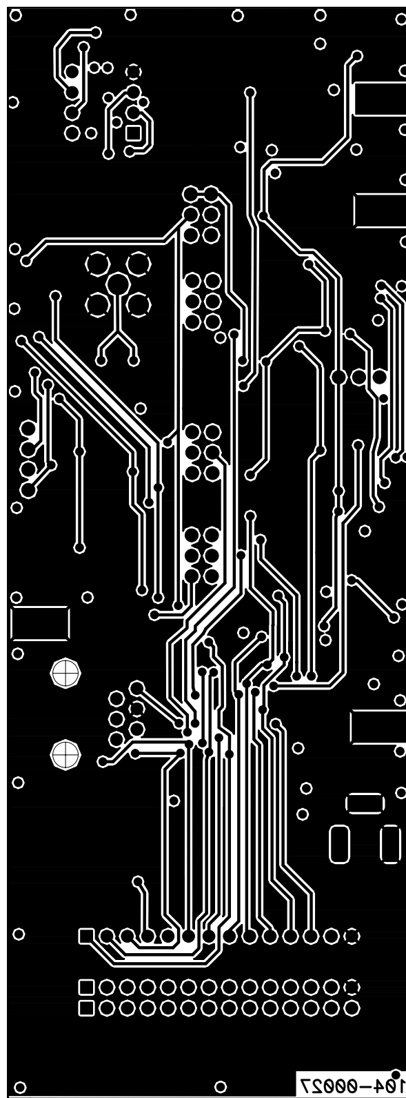
FIGURE A-5: BOARD LAYOUT - BOTTOM LAYER
