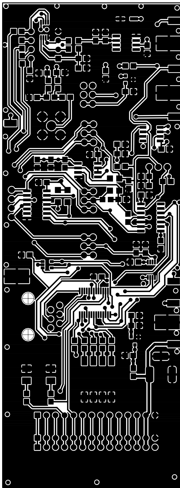
FIGURE A-4: BOARD LAYOUT - TOP LAYER
