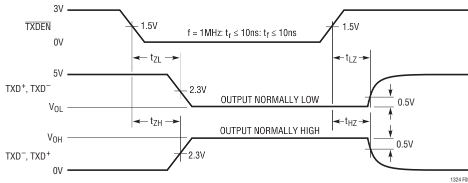
Figure 5. Differential Driver Enable and Disable
