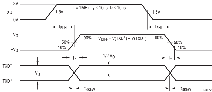
Figure 4. Differential Driver
