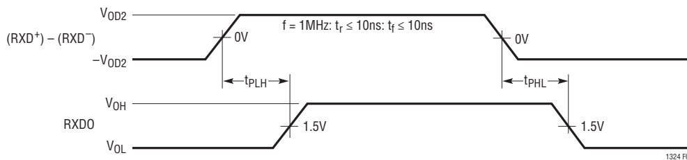
Figure 6. Differential Receiver
