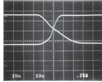
Figure 11. Low Slew Rate Mode
