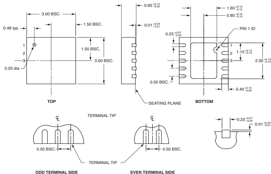
10-Pin MLF™ (ML)
