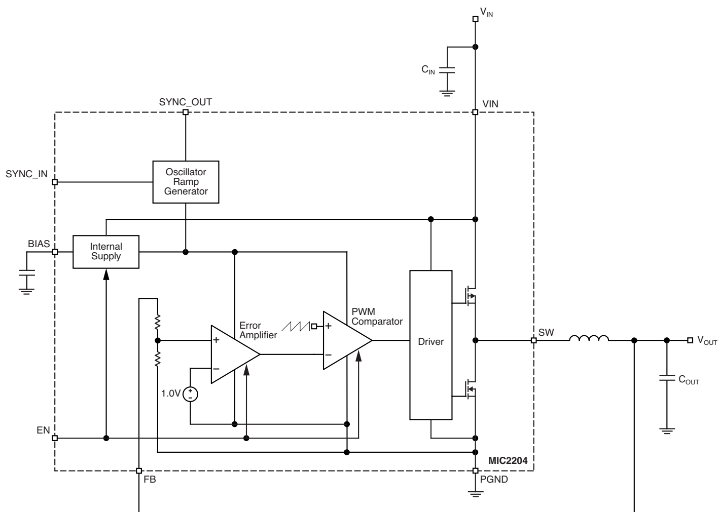
MIC2204 Block Diagram
