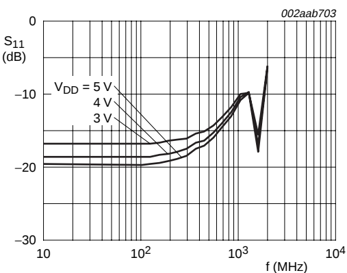
Fig 11. Input match ON-channel versus frequency and V DD
