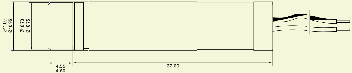
VM Fitted With External Optic
