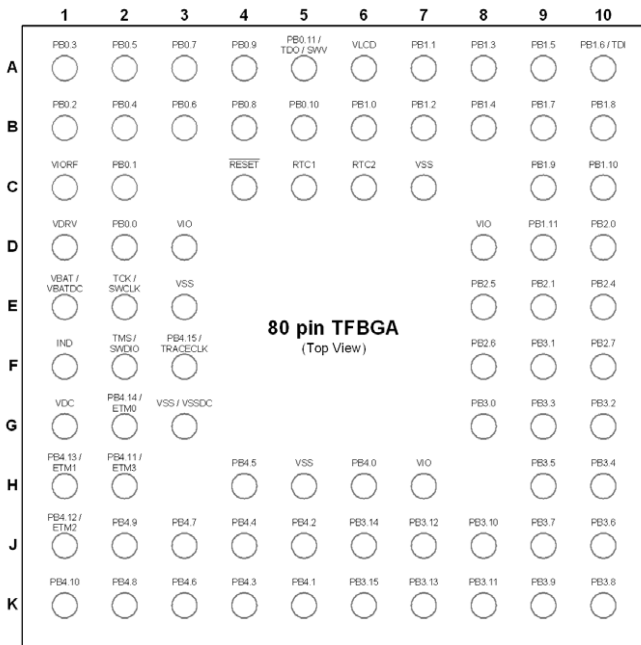
Figure 6.2. SiM3L1x7-GL Pinout
