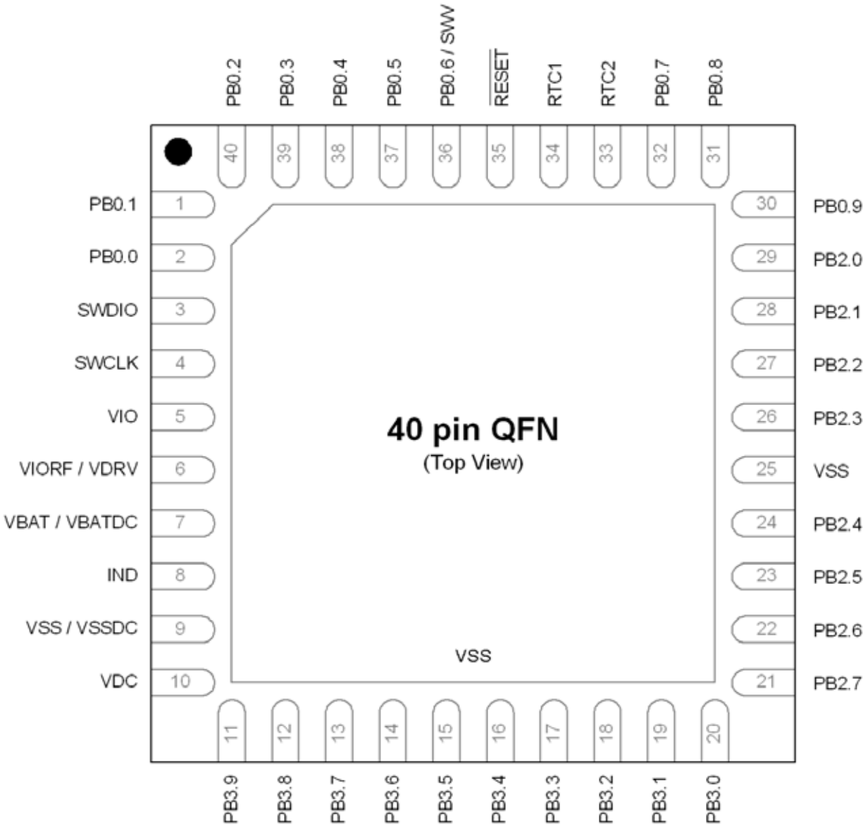
Figure 6.5. SiM3L1x4-GM Pinout
