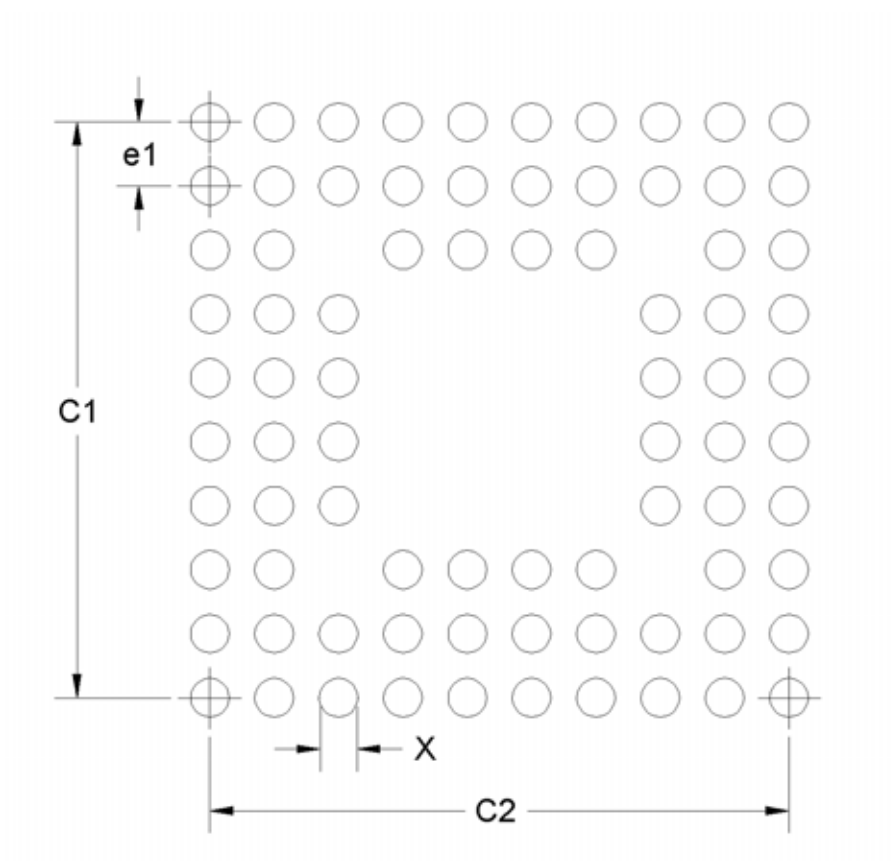
Figure 6.9. TFBGA-80 Landing Diagram
