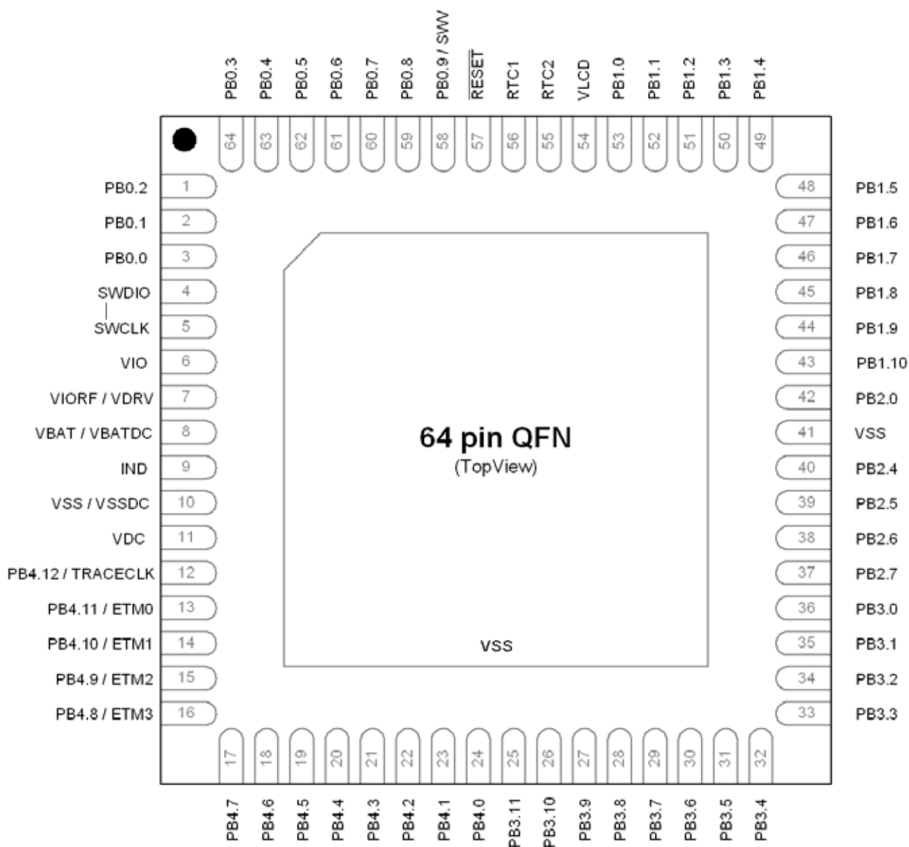
Figure 6.4. SiM3L1x6-GM Pinout
