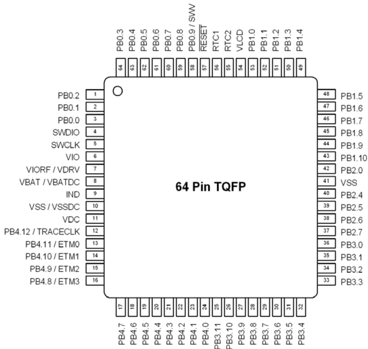
Figure 6.3. SiM3L1x6-QG Pinout
