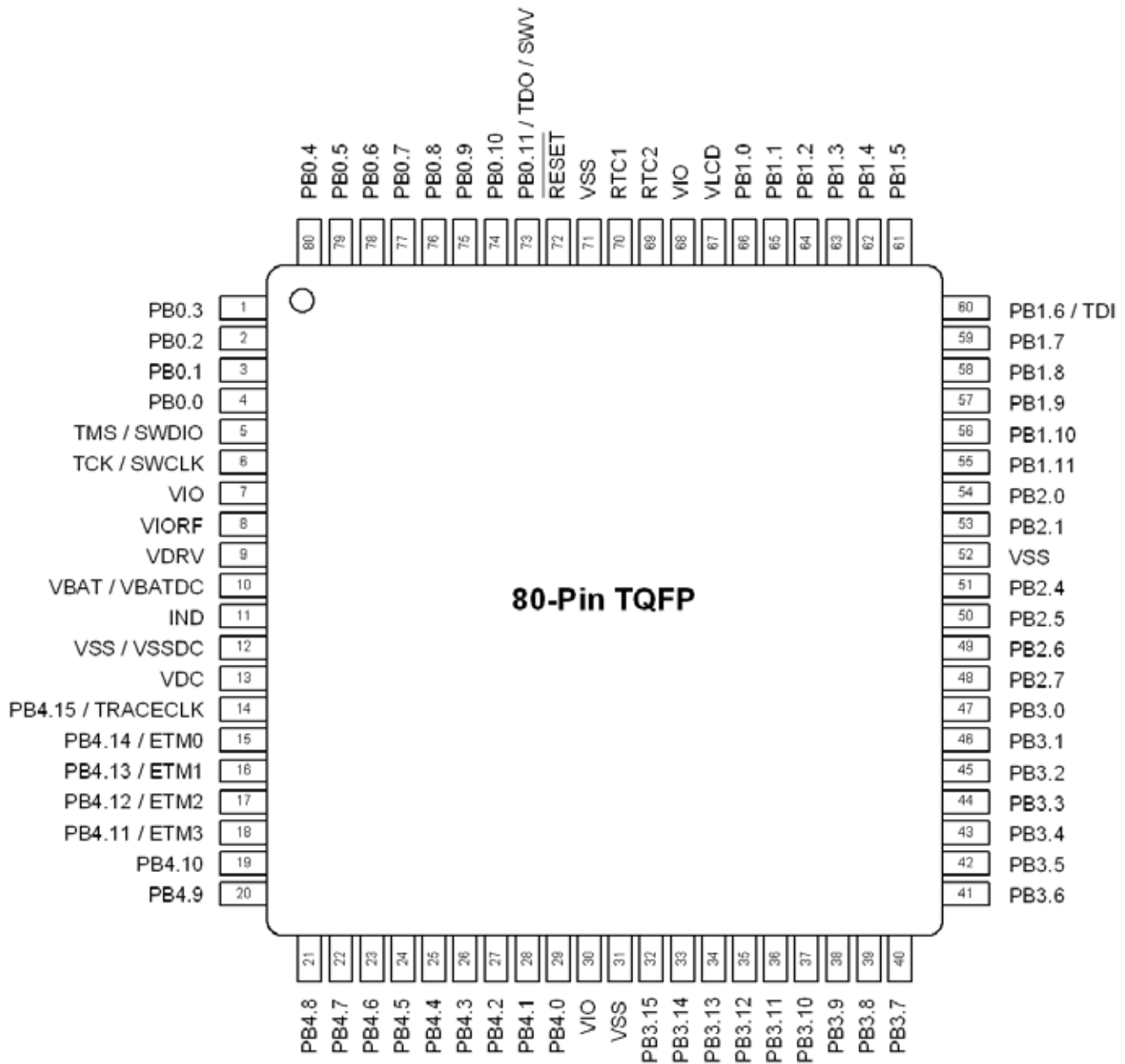
Figure 6.1. SiM3L1x7-GQ Pinout
