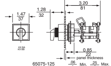
Double Pot Potentiometer Operator
