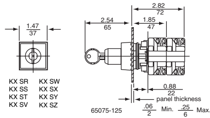
Key Operator Selector Switch
