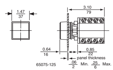
Four Lamp Pilot Light
