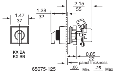
Single Pot Potentiometer Operator
