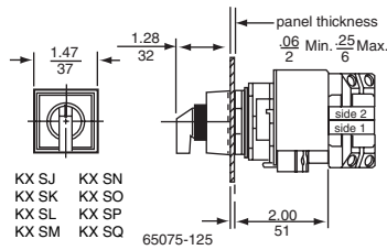
Selector Switch Operator Illuminated
