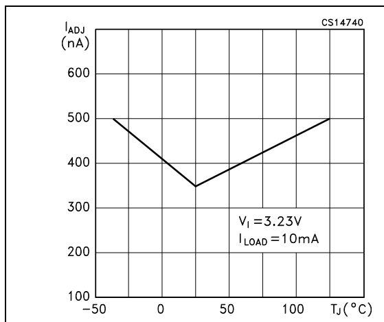
Figure 15. Adjust pin current vs. temperature
