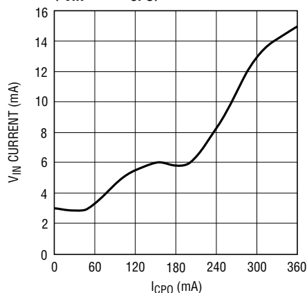
1.5x Mode V_{IN} Current vs I_{CP0} ( I_{VIN} - 1.5I_{CP0} )
