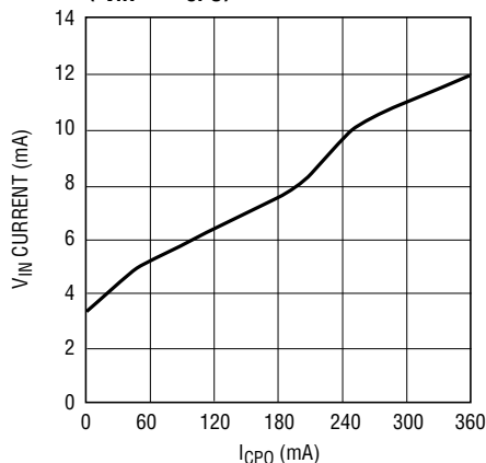
2x Mode V_{IN} Current vs I_{CP0} ( I_{VIN} - 2I_{CP0} )
