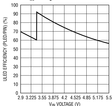
18-LED ULED Display Efficiency vs V_{IN} Voltage
