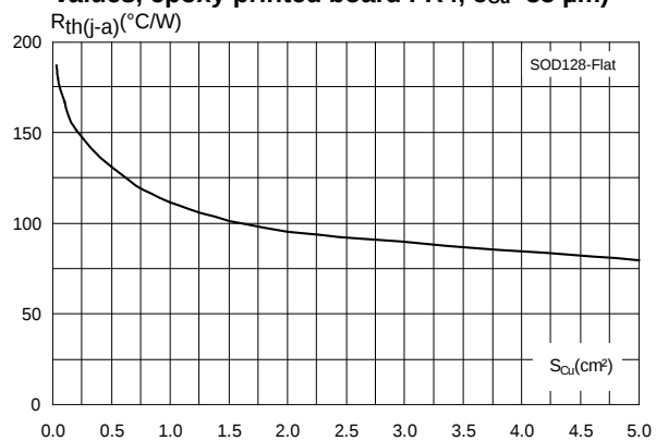
Figure 8: Thermal resistance junction to ambient versus copper surface under each lead (typical values, epoxy printed board FR4, e_{Cu}=35\text{ }\mu\text{m} )
