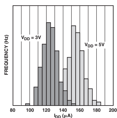
Figure 10. I_{DD} Histogram with V_{DD} = 3\text{ V} and V_{DD} = 5\text{ V}
