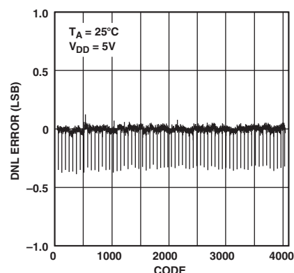
Figure 7. AD5321 Typical DNL Plot
