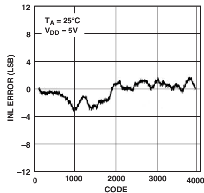
Figure 4. AD5321 Typical INL Plot
