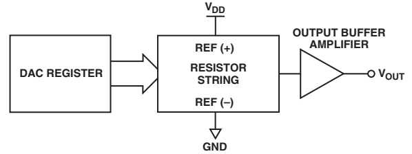
Figure 21. DAC Channel Architecture
